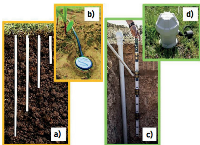
Soil sensors Drill and Drop (a,b) Enviroscan (c,d). Photograph: Gaia Sense
